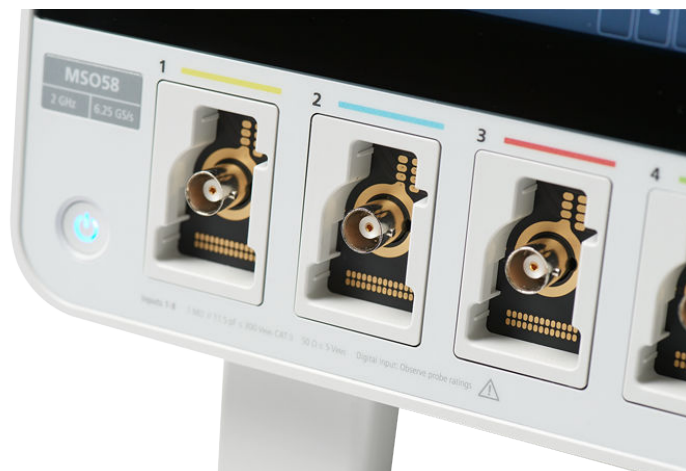
FlexChannel technology enables the ultimate in flexibility. Each input can be configured as a single analog or eight digital channels based on the type of probe you attach.
