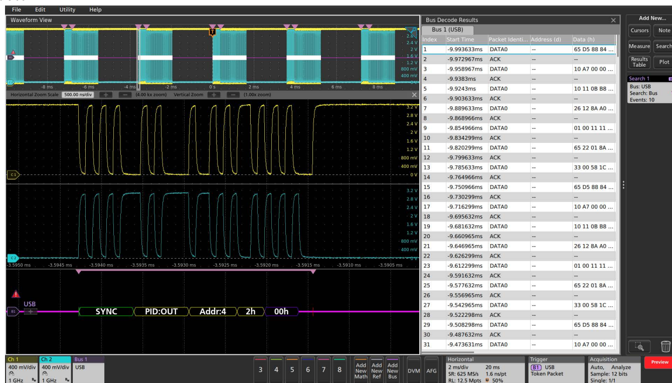
Triggering on a USB full-speed serial bus. A bus waveform provides time-correlated decoded packet content including Start, Sync, PID, Address, End Point, CRC, Data values, and Stop, while the bus decode table presents all packet content from the entire acquisition.
